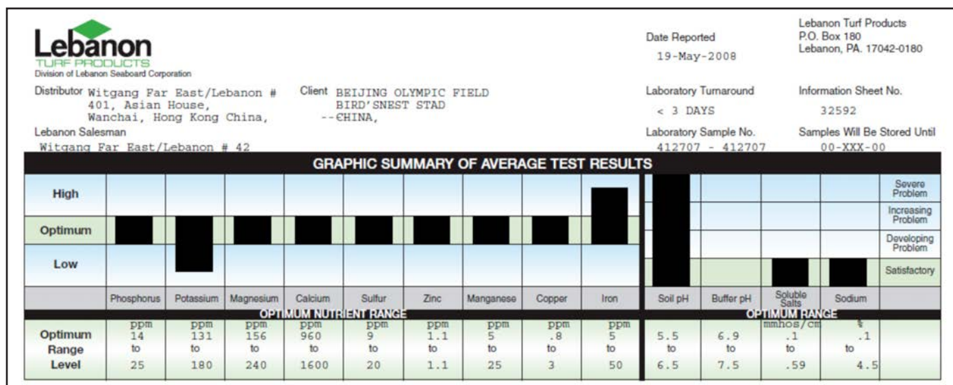
Figure 3: A "Complete Soil Test" will include soil pH, the macronutrient; phosphorus (P), potassium (K), magnesium (Mg), calcium (Ca), sulfur (S), and micronutrients; iron (Fe), zinc (Zn), copper (Cu), manganese (Mn) and sodium (Na).
